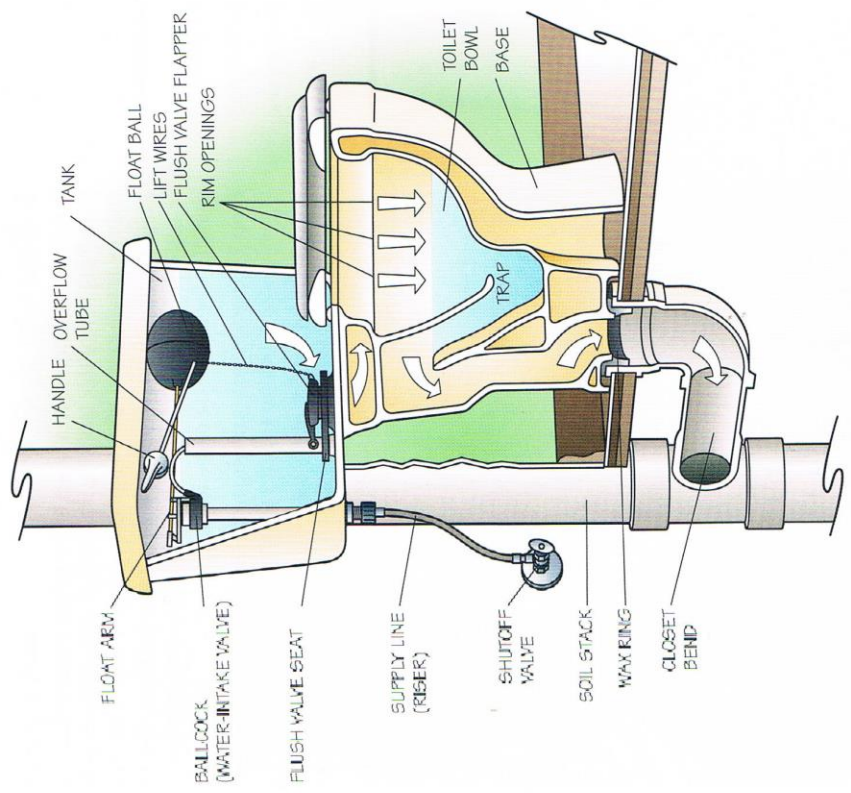
A gravity-assist flush toilet with a float ball
